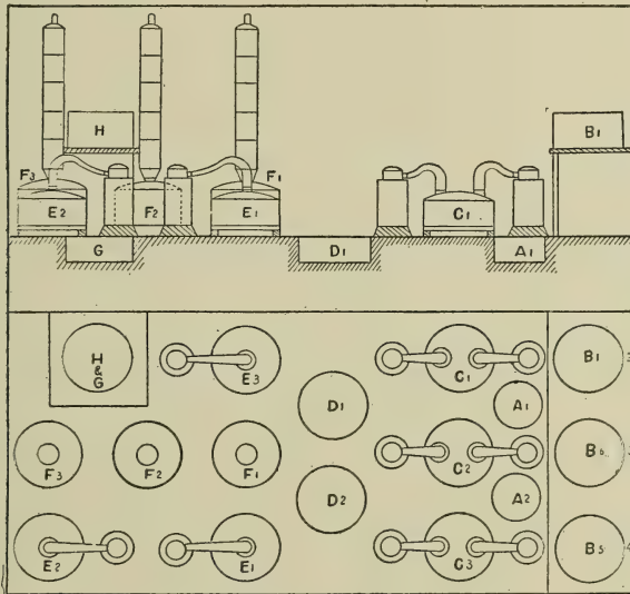
FIG. 77.—Plant for Refining Wood Tar.
